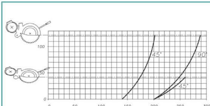
Rezný diagram NORMA 400
