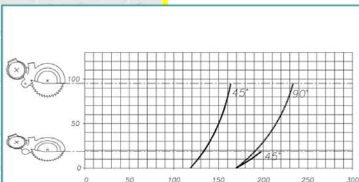
Rezný diagram NORMA 350
