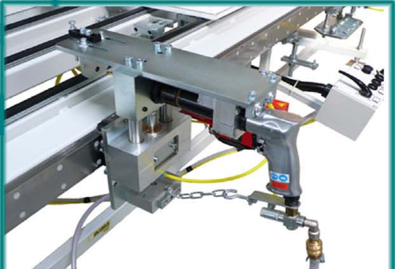
Movable drilling unit
